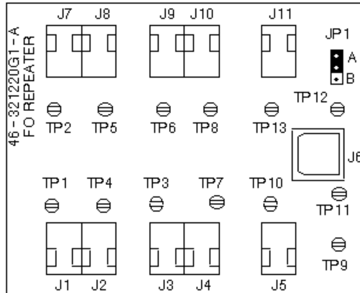
FIBER OPTIC REPEATER BOARD ILLUSTRATION L2520A
